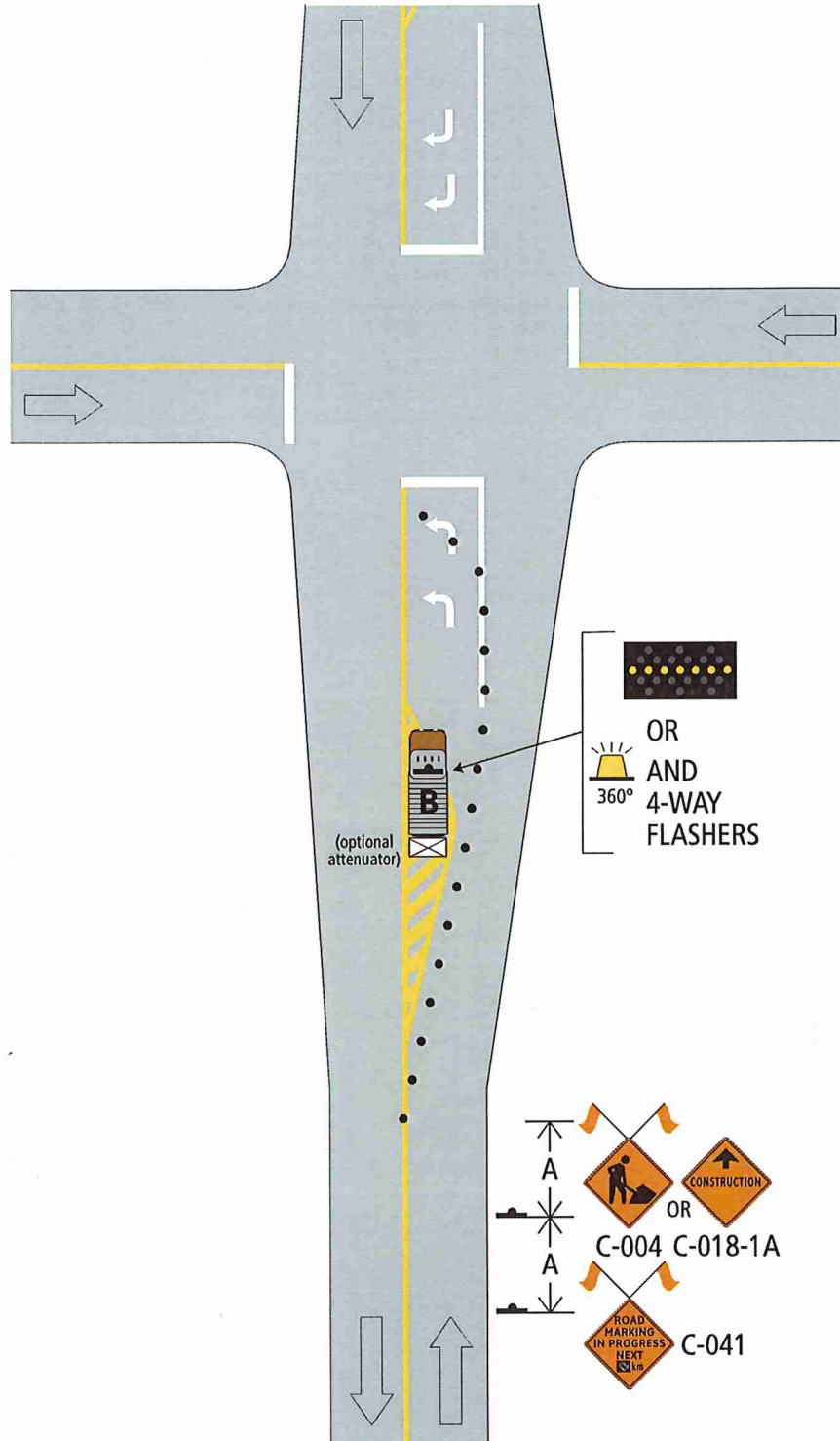
Figure 14.9: Left-Turn Arrow Marking – Short and Long Duration
